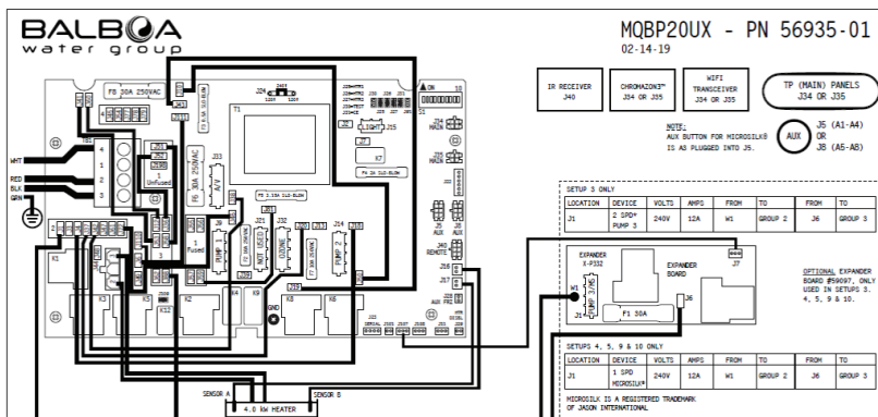
Wiring Diagram
